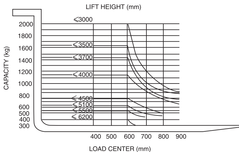
MAST DETAILS FOR ELECTRIC STACKER (ES Model)
